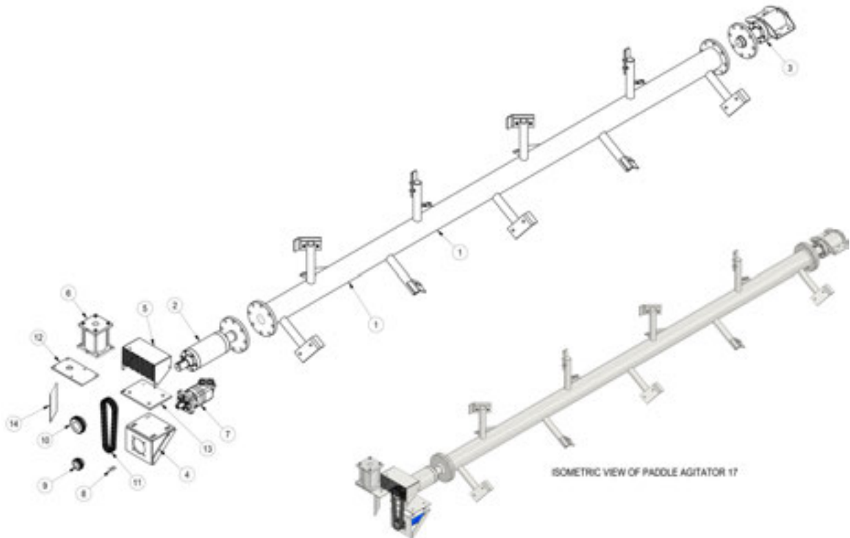
BOM OF PADDLE AGITATOR FULL ASSEMBLY
